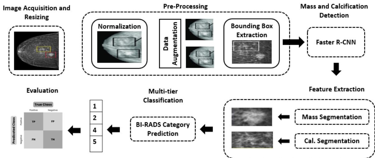
Figure 6. A multi-label classification framework for BI-RADS category prediction
